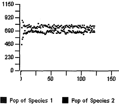
Figure 2.3 population vs time
