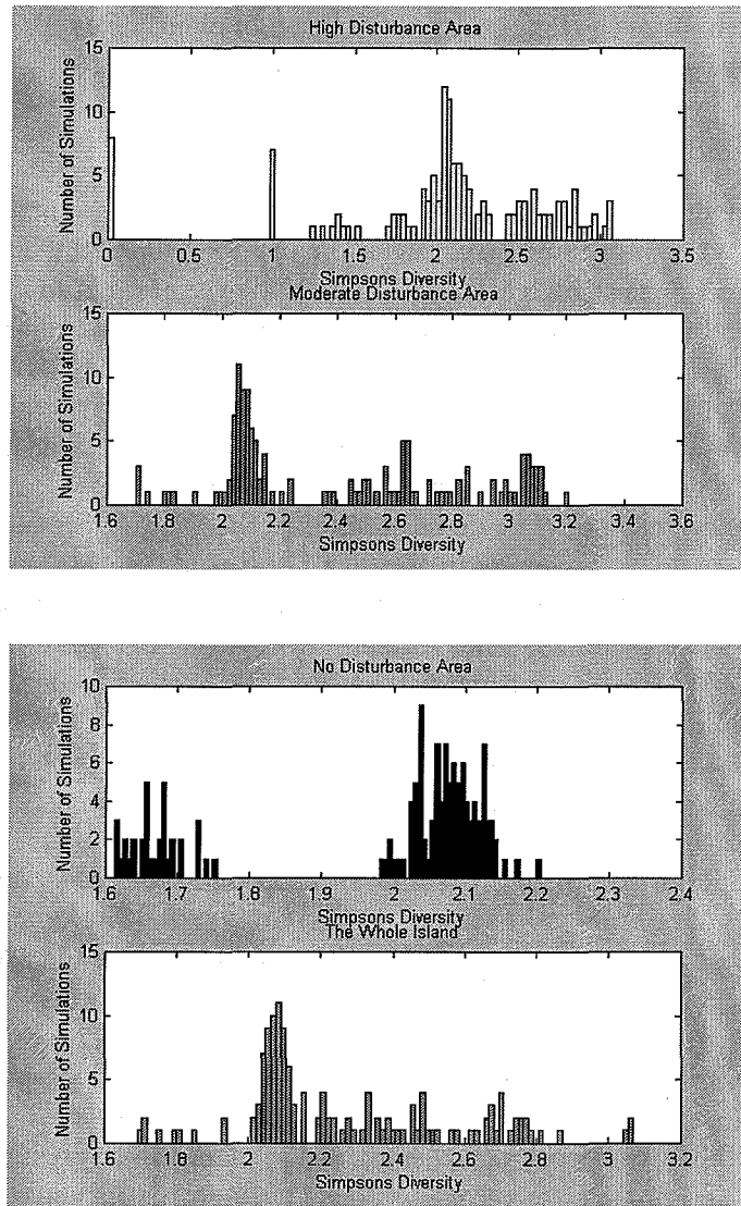
Figure 7.2: Histograms for Different Levels of Disturbance
