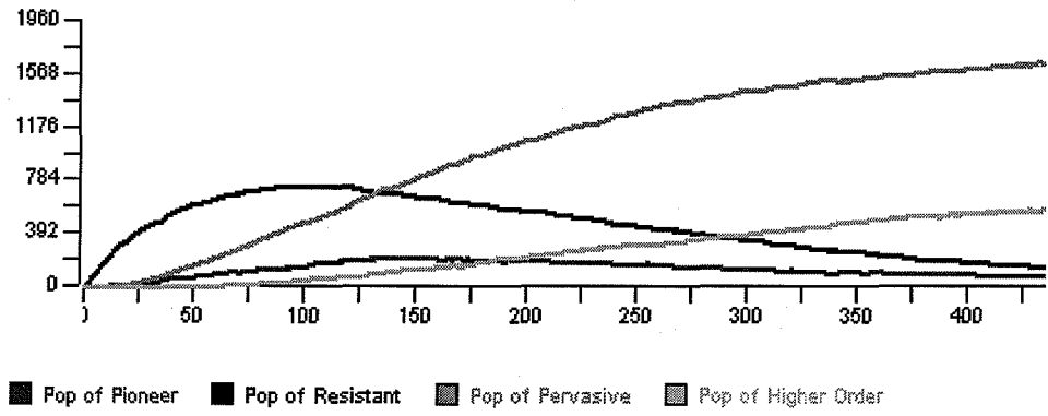
Figure 4.4 The recovery of plant species with no periodic disturbance (population vs time)
